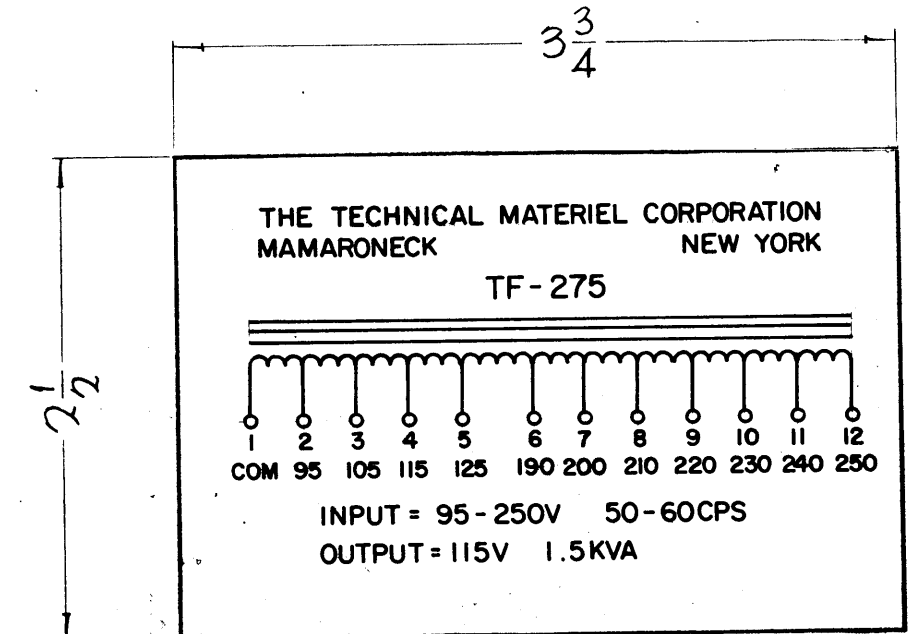
NAMEPLATE DETAIL
