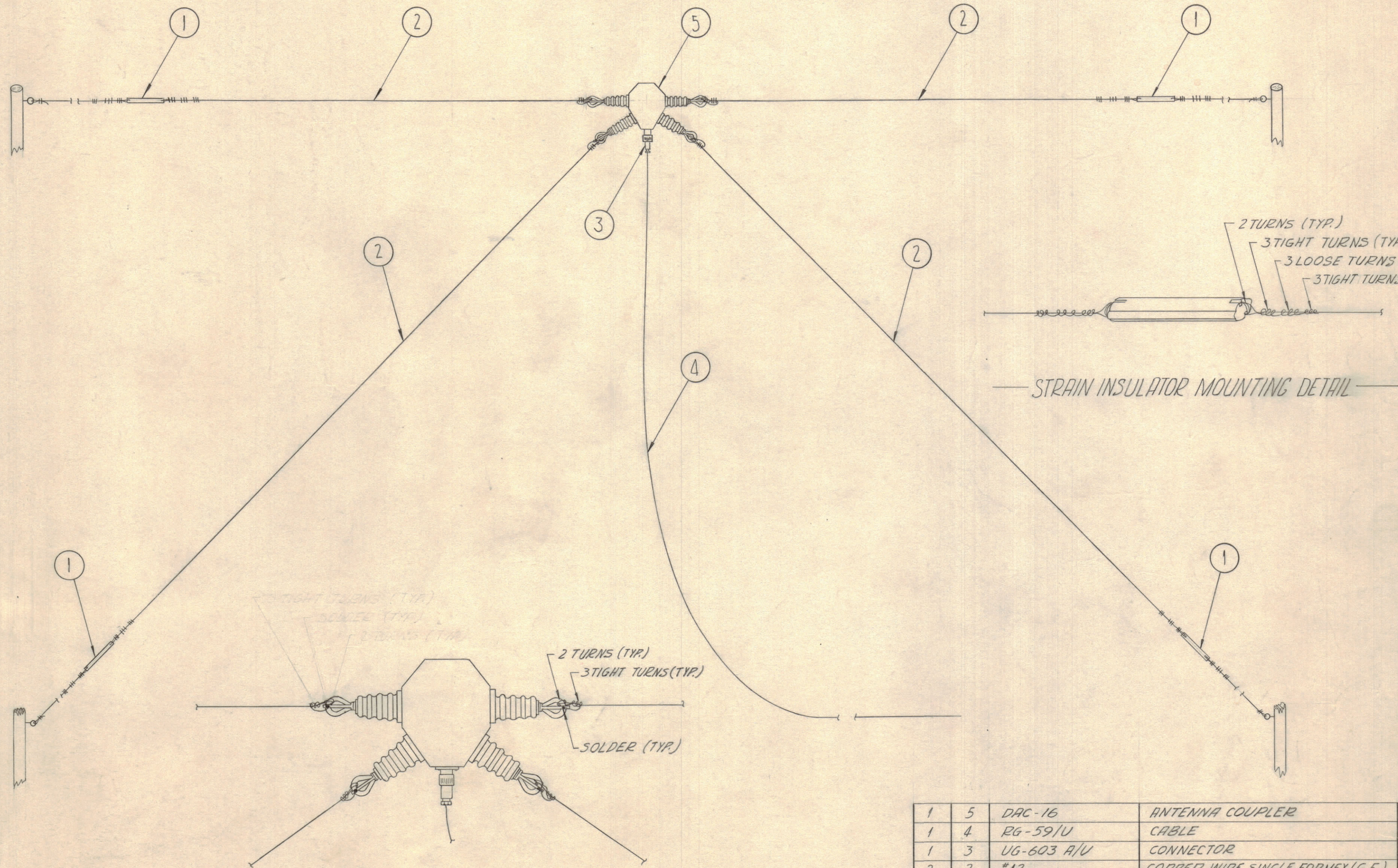
—DAC-16 MOUNTING DETAIL—
