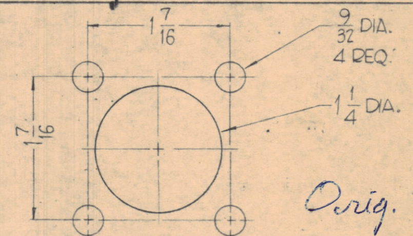
DETAIL "E" (2 REQ)
