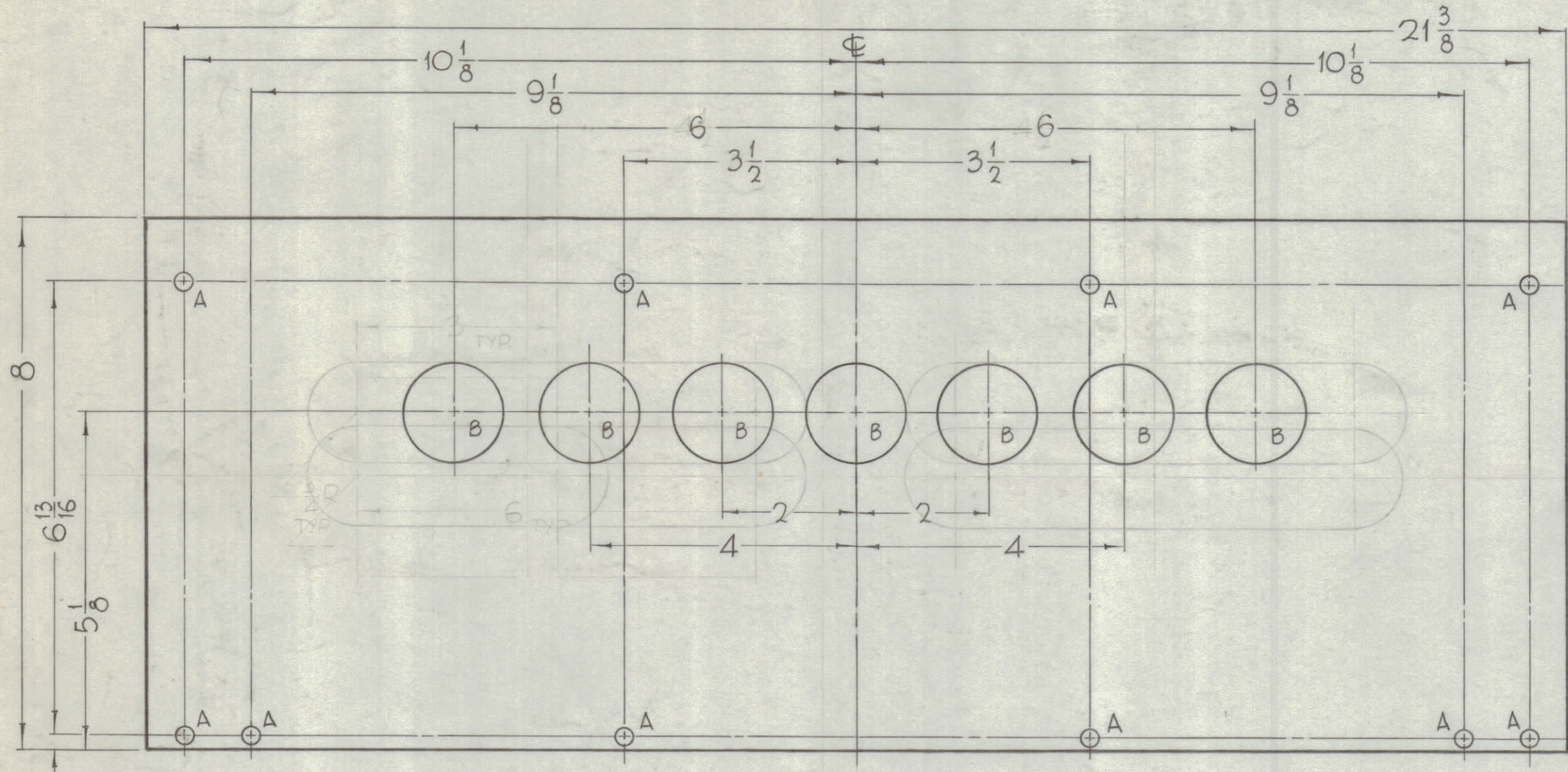
PX-770-1 (4 REQ.)
