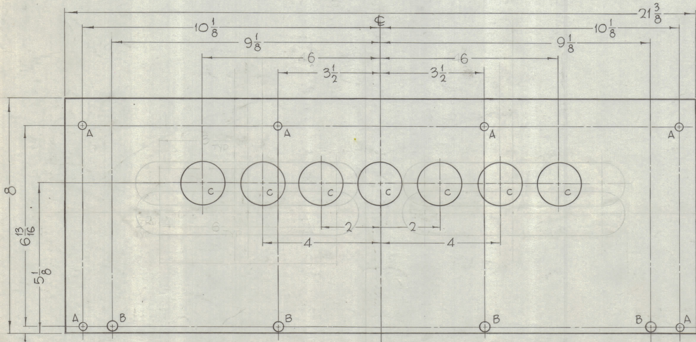
PX-770-2 (2 REQ.)
