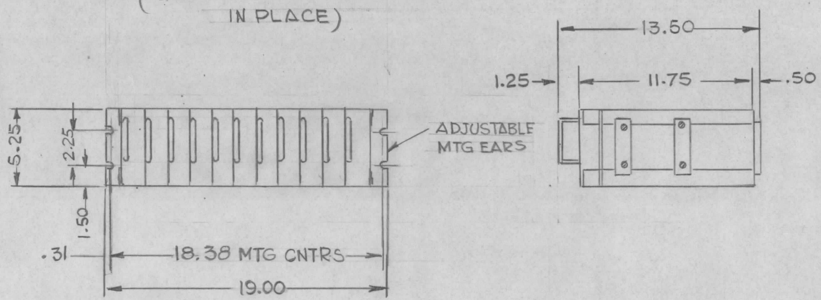
FRONT VIEW (SHOWN WITH MODULES IN PLACE)
