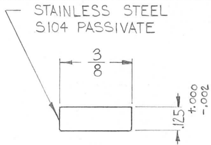
"B" DETAIL
