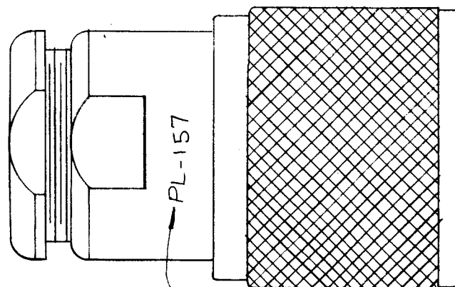
METAL STAMP TMC PART NO AS SHOWN 1/16 HIGH GOTHIC.
