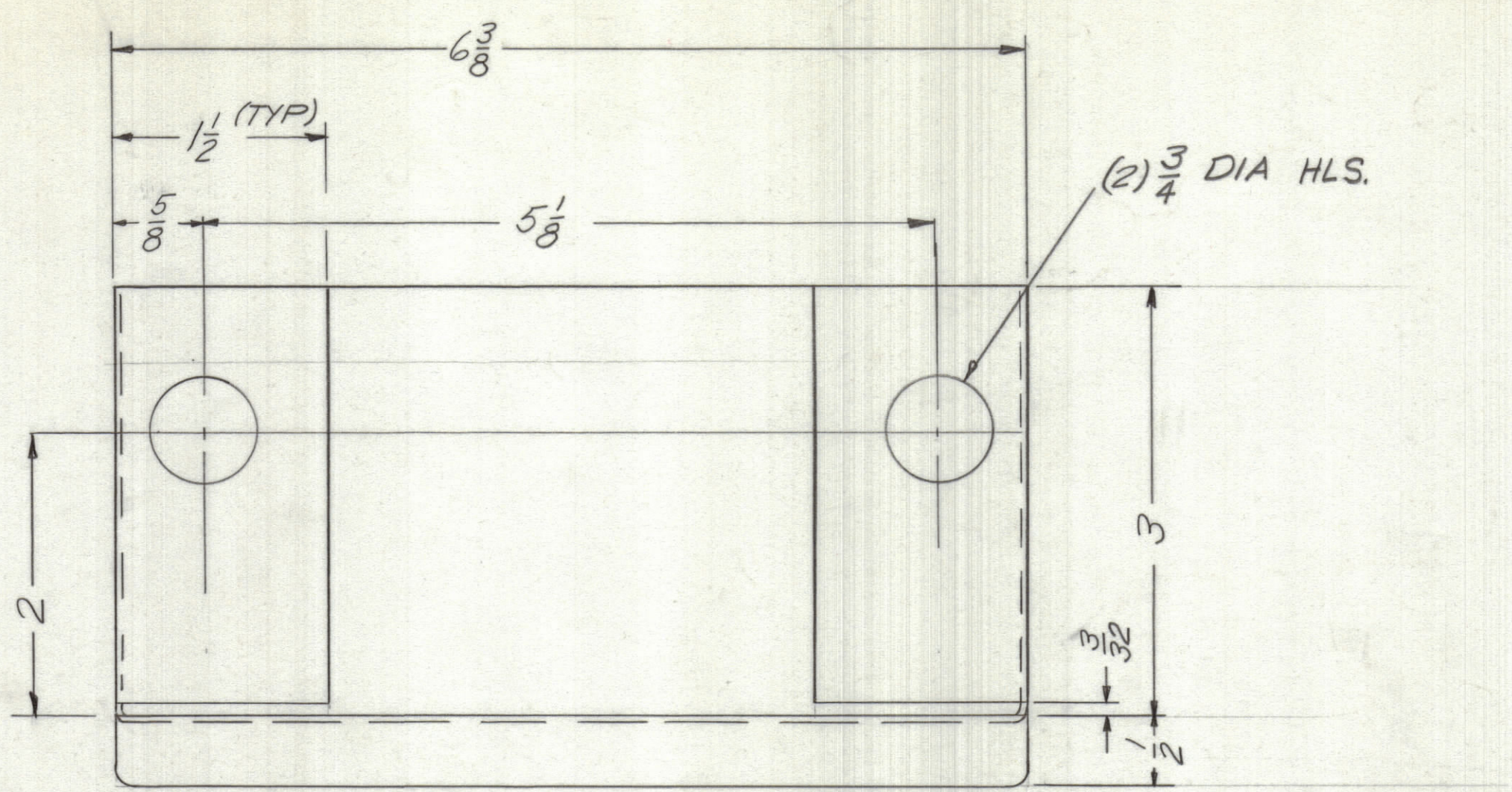
END VIEW A-A
