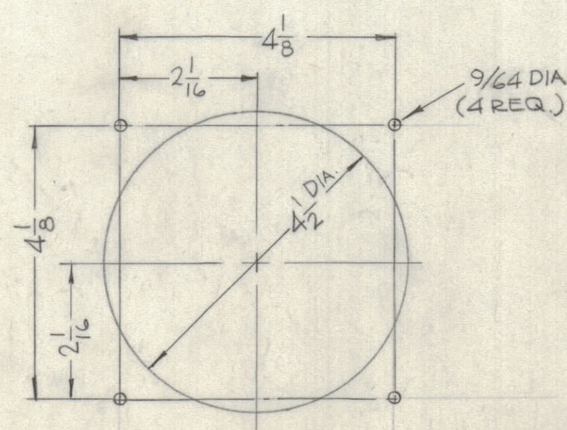
DETAIL - B
