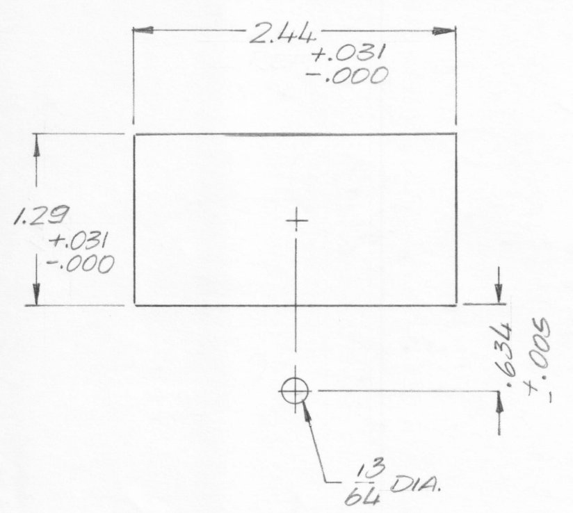
PANEL MOUNTING DIMENSIONS
