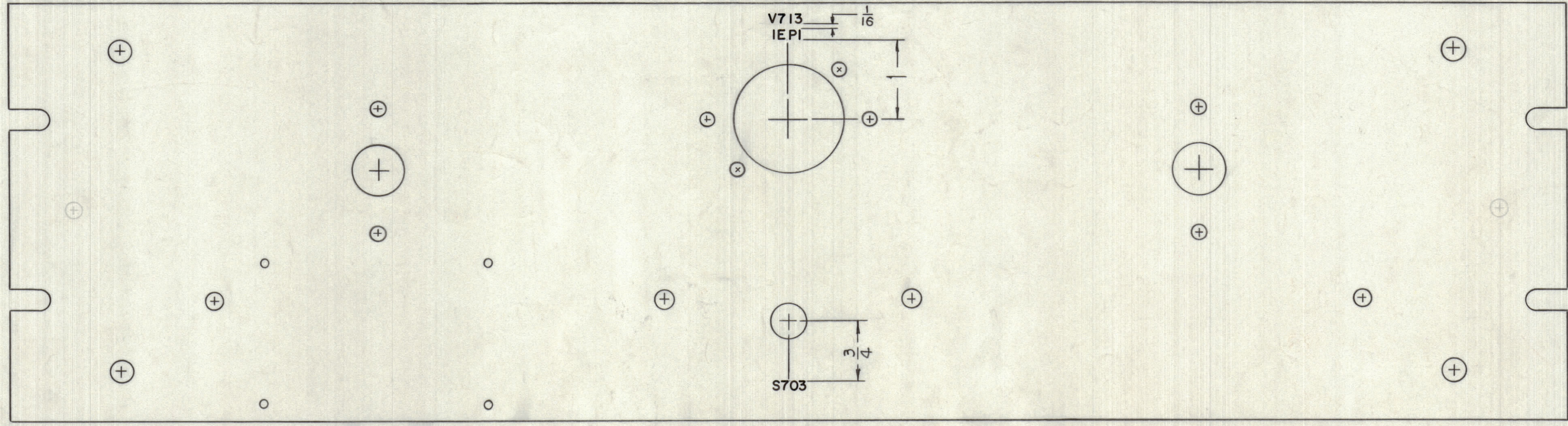
REAR VIEW OF PANAL SHOWN (TO BE SILK SCREENED) OR EQUIVALENT PER TMC SPEC-S 544
