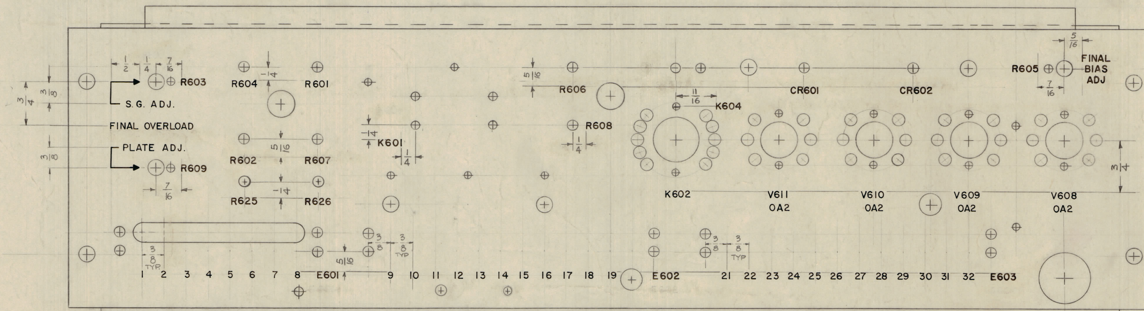
TOP VIEW
