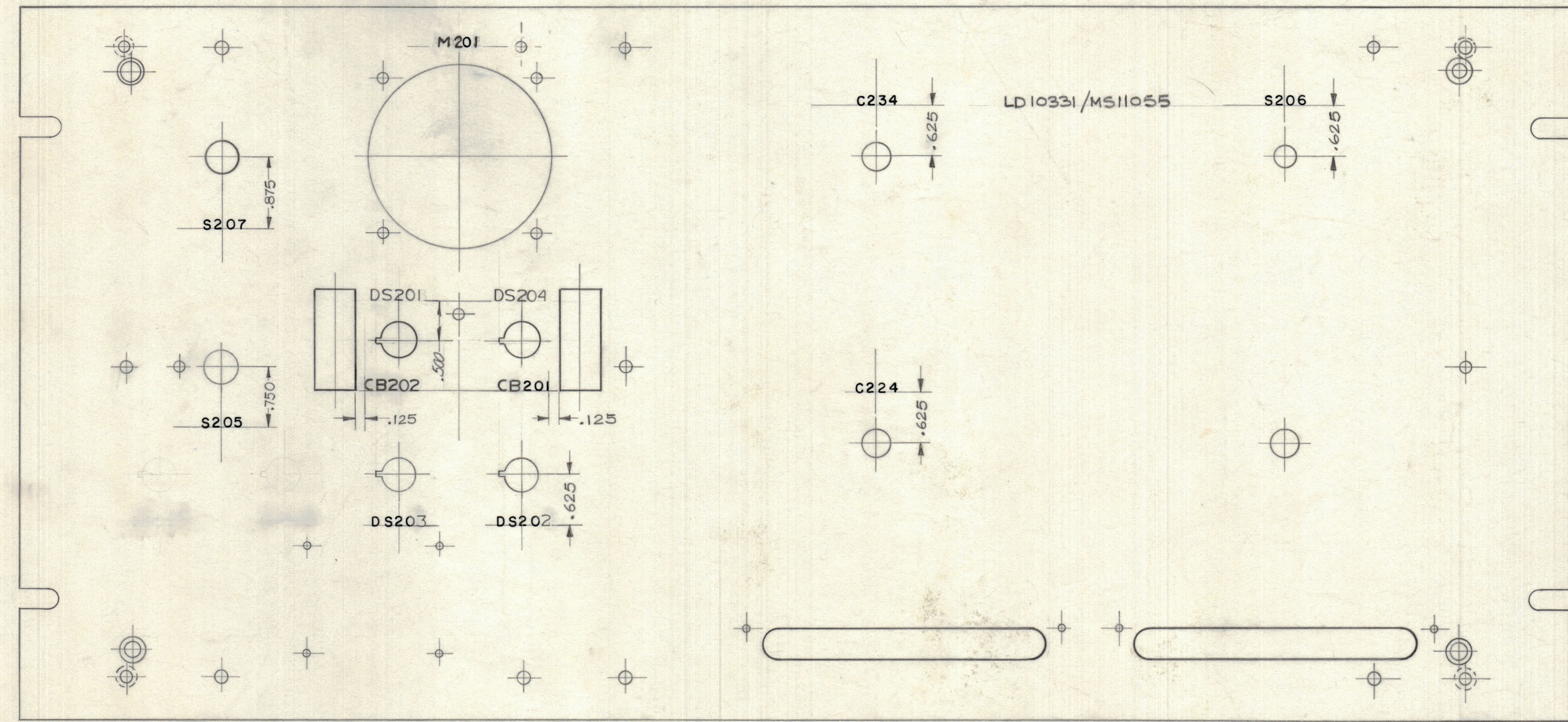
REAR VIEW OF FRONT PANEL
