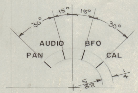
MONITOR ANGLE DISPLACEMENT
