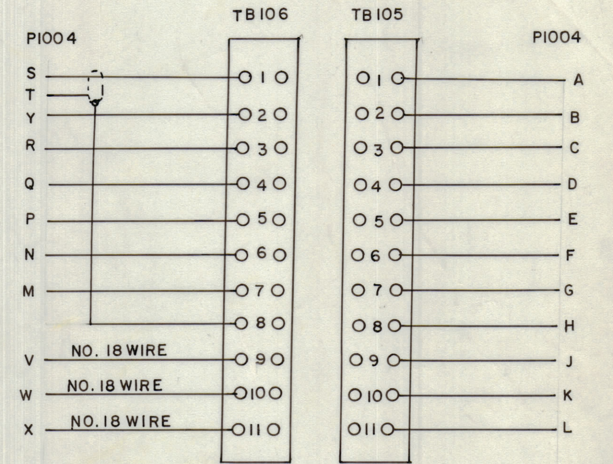
ANTENNA TUNER INTER CONNECT CABLE WIRING
