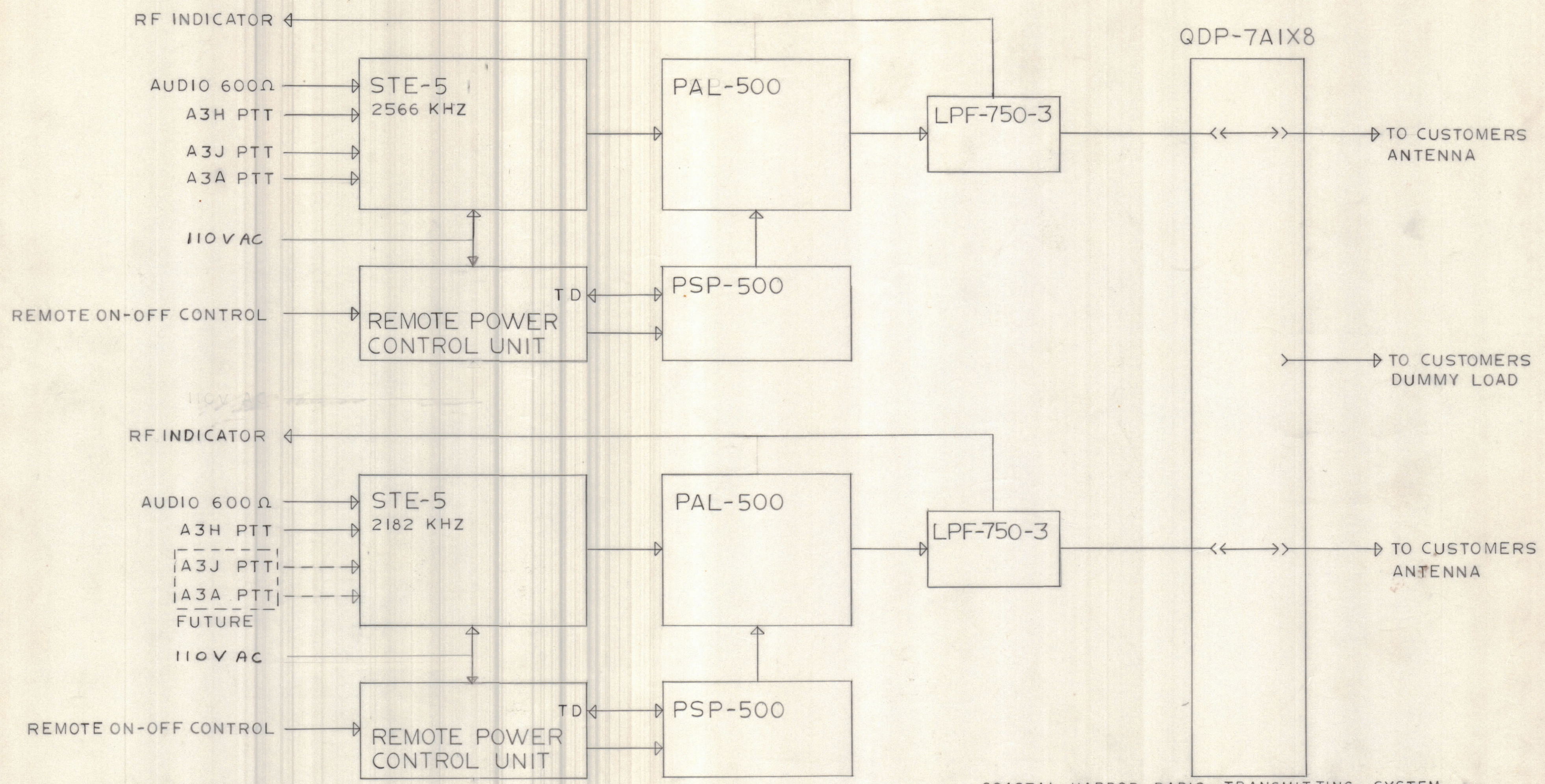
COASTAL HARBOR RADIO TRANSMITTING SYSTEM KTJ
