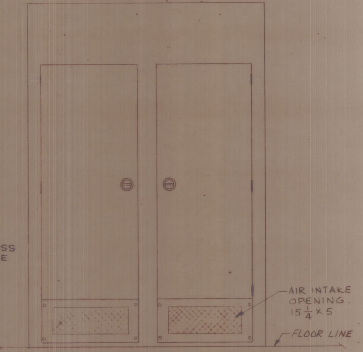
REAR VIEW
