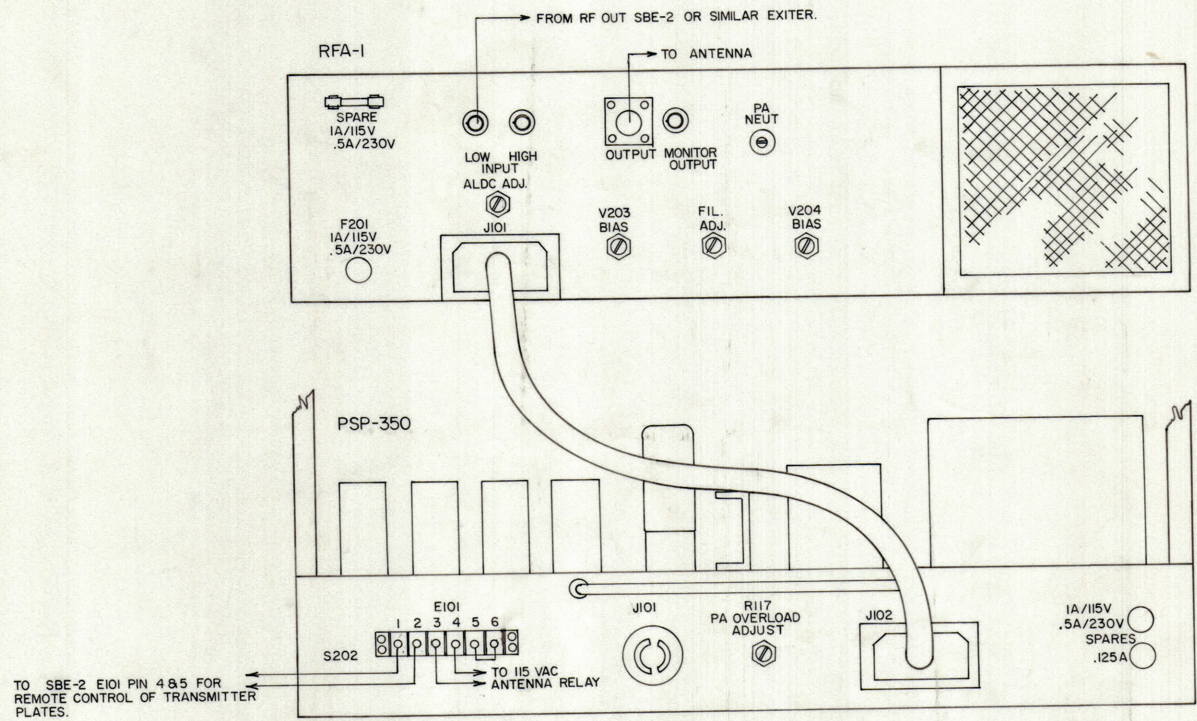
REAR PANEL CONNECTIONS & ADJUSTMENT
