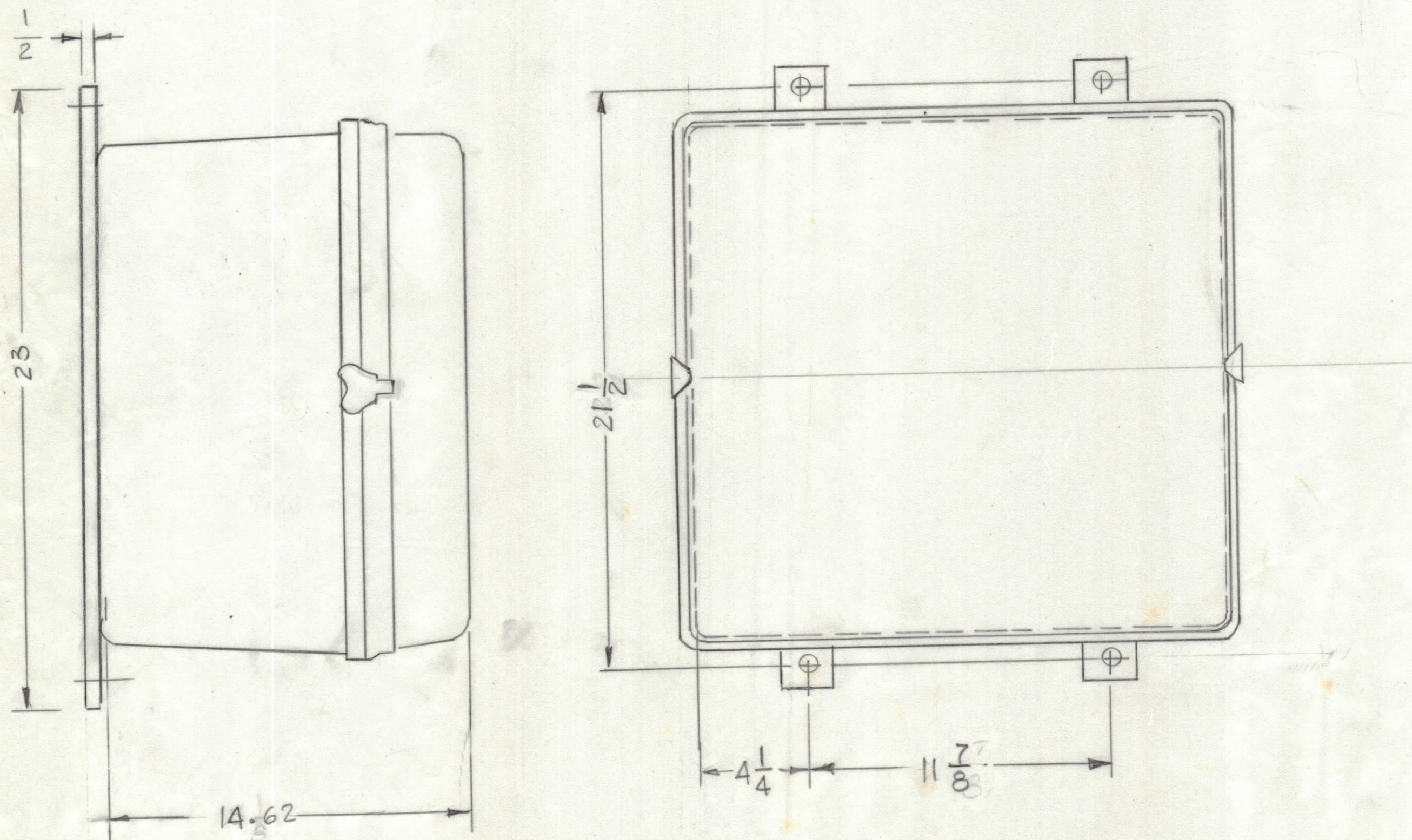
MOUNTING & OUTSIDE DIMENSION
