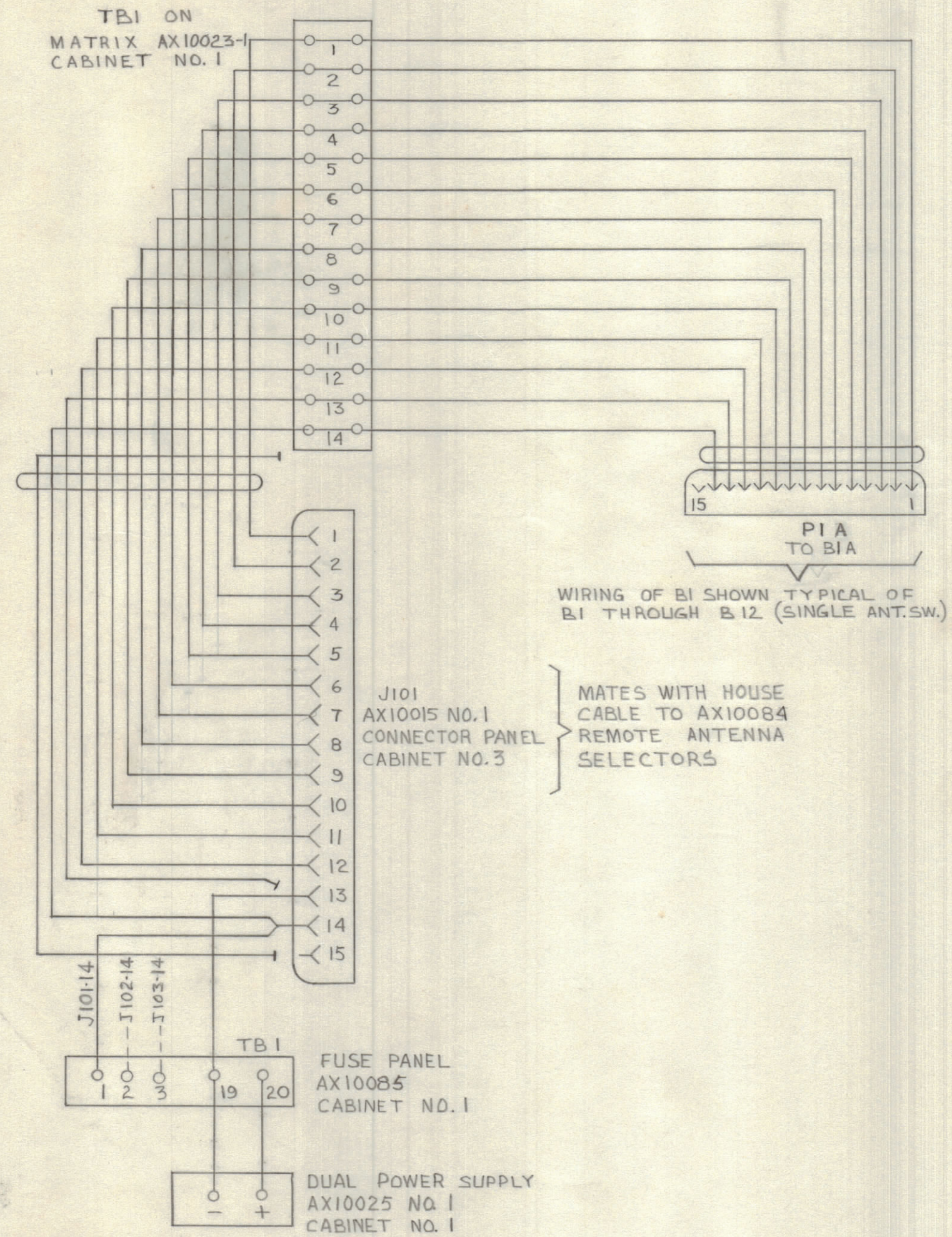
SINGLE ANTENNA SELECTION "B" CIRCUIT CABLING
