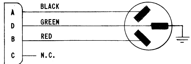
AC POWER CABLE FOR J4 ON STR-5( )
