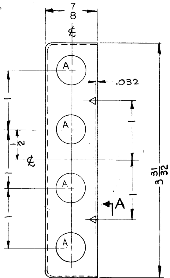
PARTIAL SECTION A-A
