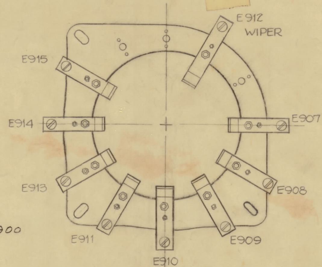
TOP VIEW OF WAFER AND CONTACTS (T-Bracket And Spacers Removed For Clarity.)
