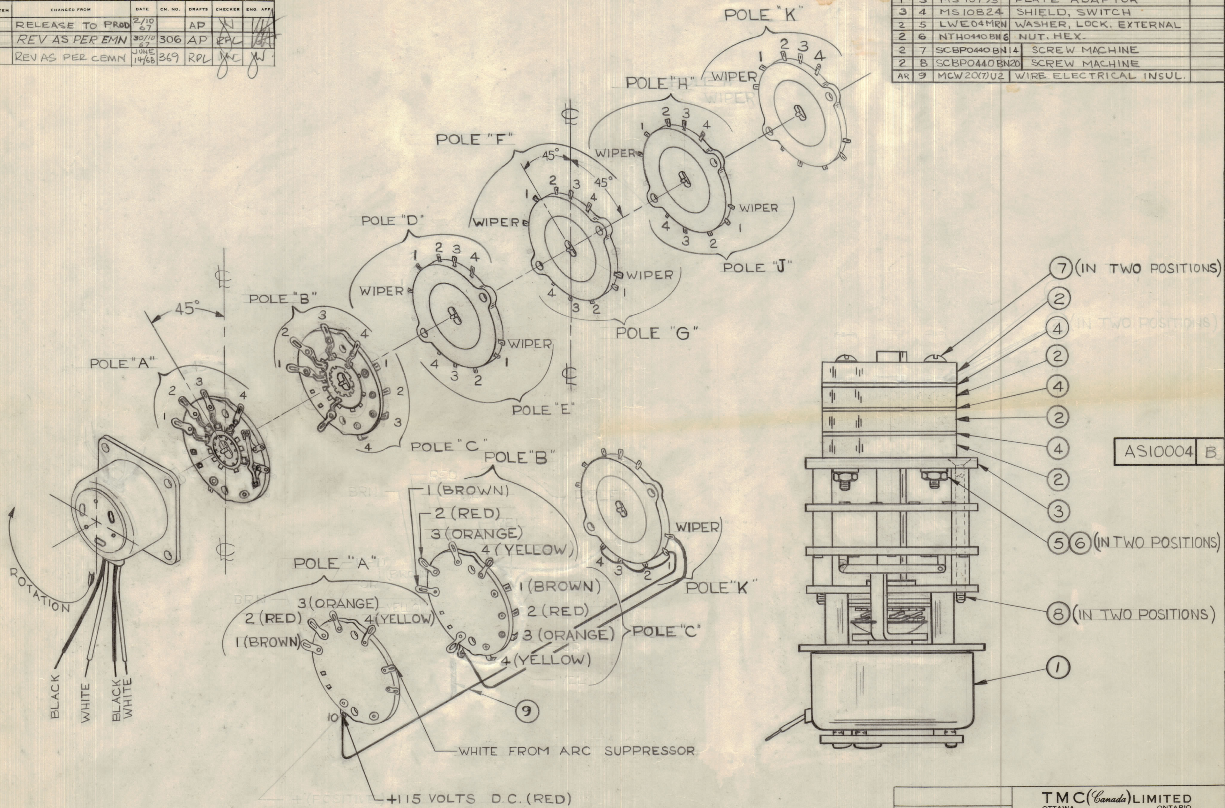
WIRING DIAGRAM OF CONTROL WAFERS
