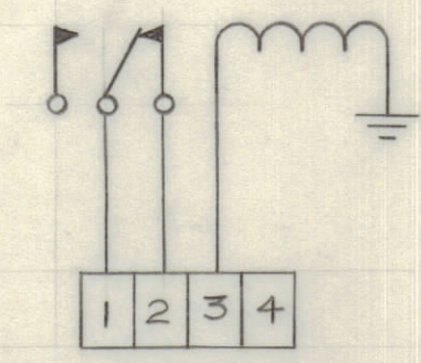
SCHMATIC NOTE: RELAY SHOWN ENERGIZED
