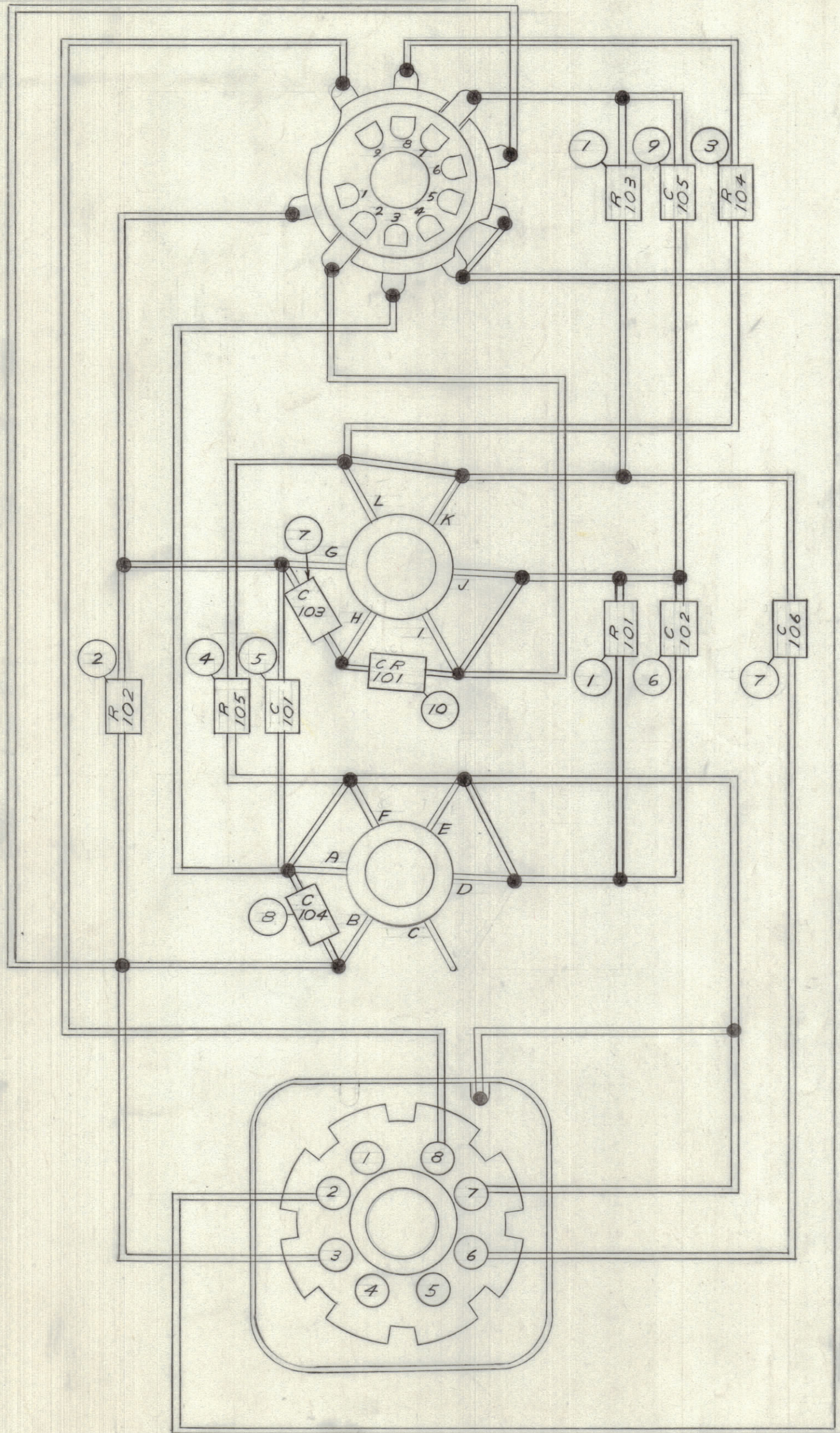
SECTION "BB"
