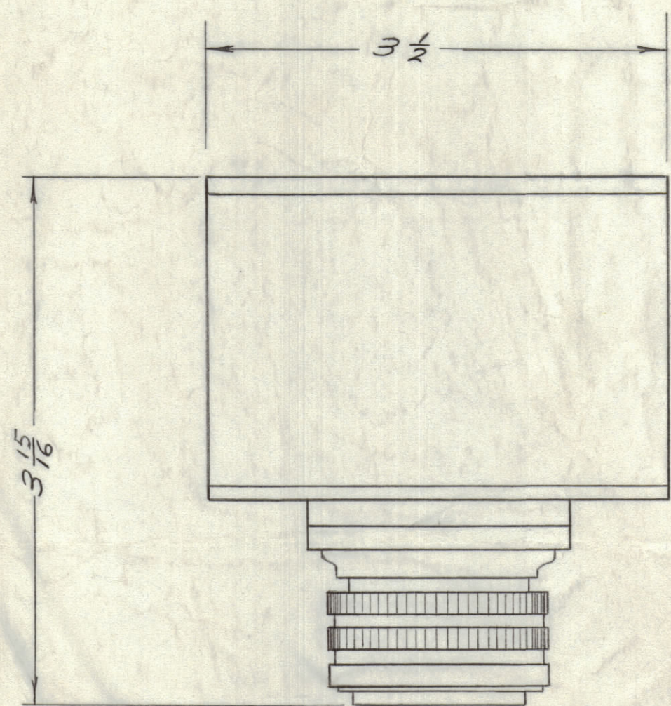
SIDE VIEW
