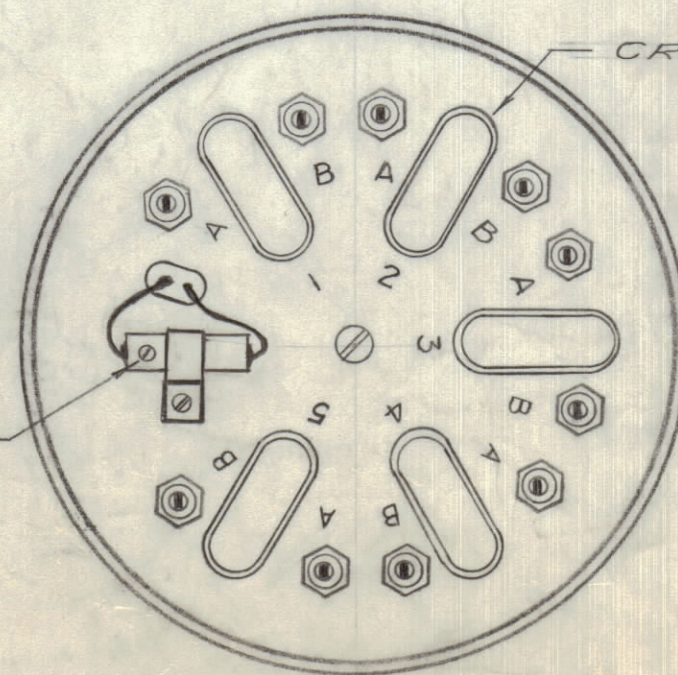
TOP VIEW WITHOUT COVER
