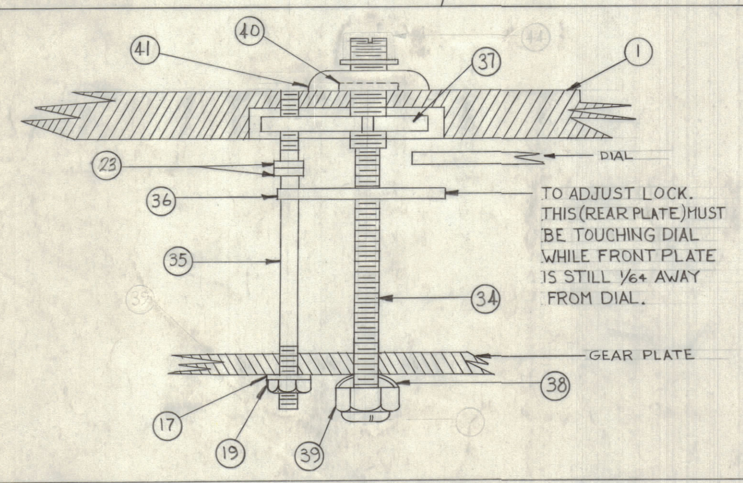
INSTALLATION & ADJUSTMENT DETAIL - DIAL LOCK ASS'Y.
